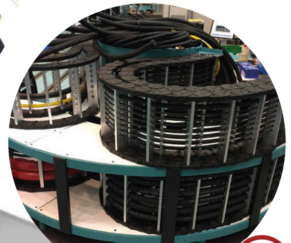
Telescope instrumentation
